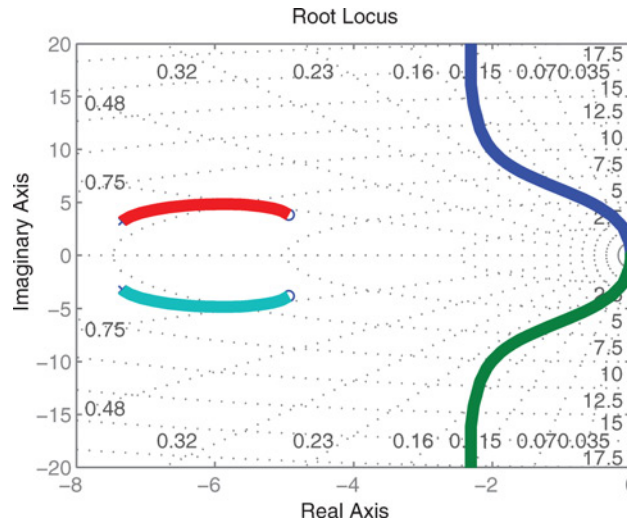
Fig. 3 Root locus plot.
