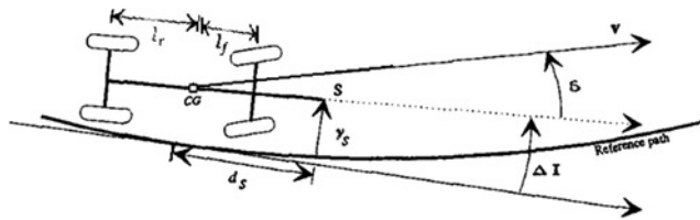
Fig. 2 Lateral vehicle dynamics.
