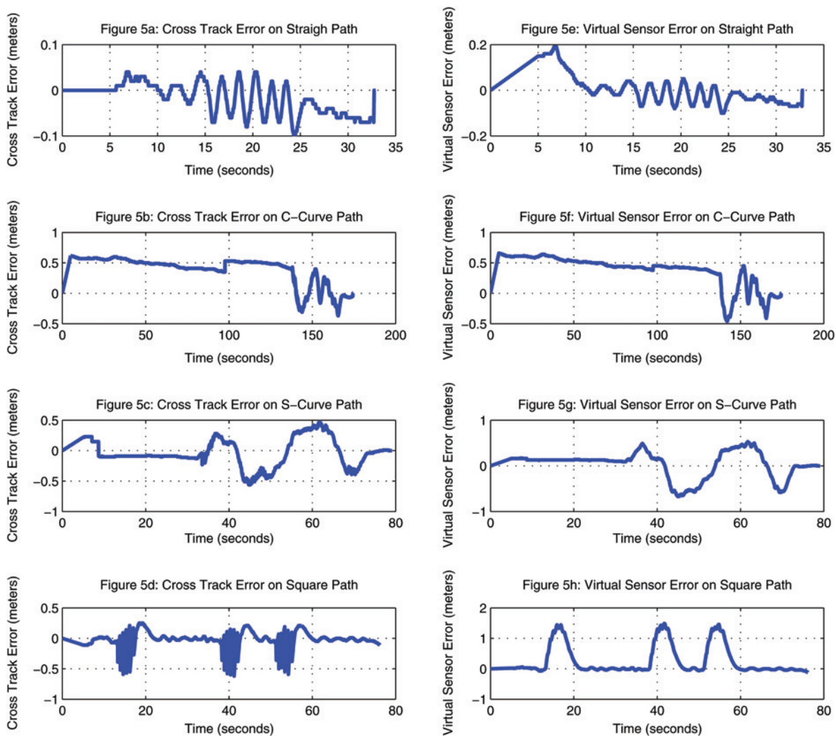
Fig. 5 Cross-track error and virtual sensor error for various paths.
